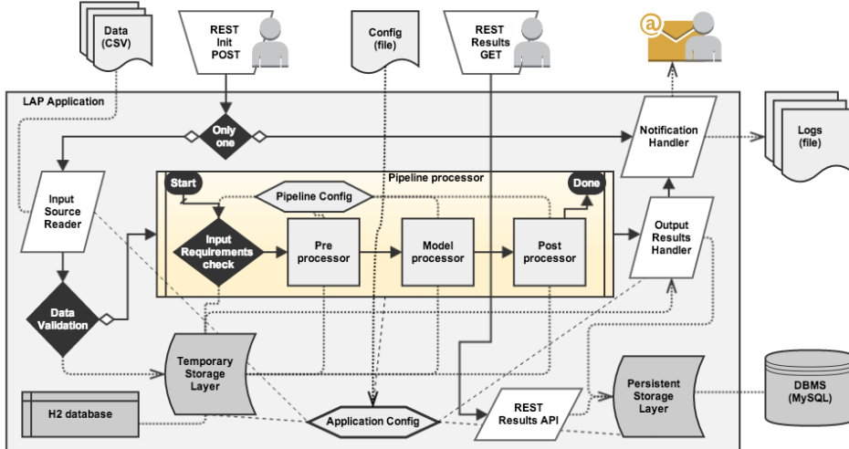
Learning Analytics Processor Architecture Diagram - Initial
