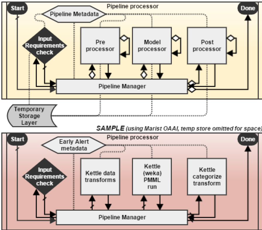
Learning Analytics Processor Pipeline Diagram - Initial
